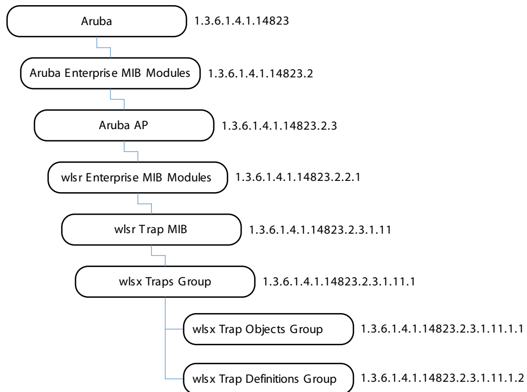
Figure 16 Trap Hierarchy
